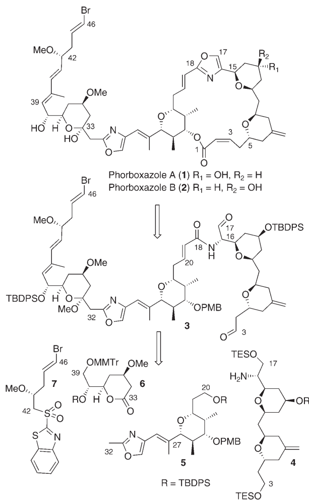
Scheme 1. Phorboxazole retrosynthesis. Protecting groups are defined in Scheme 2.
